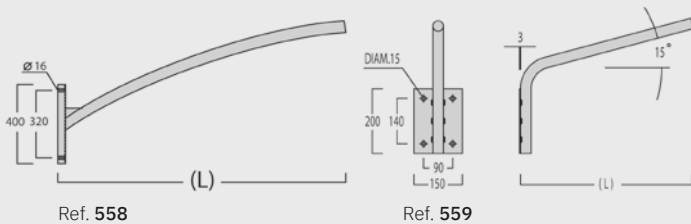
Refs. 558-559 Brazos de pared Arco
